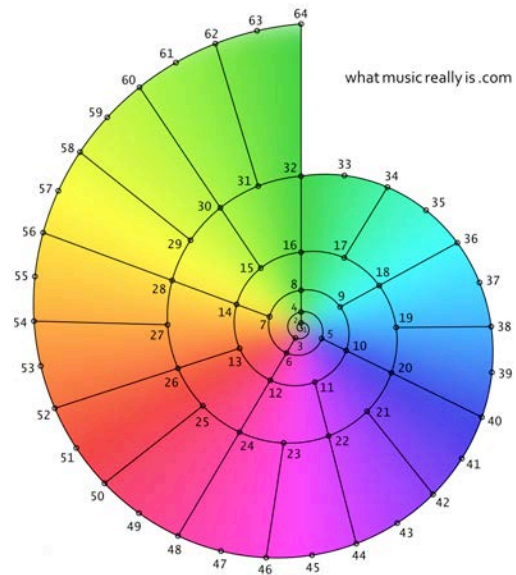
THE HARMONIC SERIES AS A LOGARITHMIC SPIRAL Issued by Erv Wilson March 1, 1965 Vector graphics and colors by Bo Constantinsen March 2015
